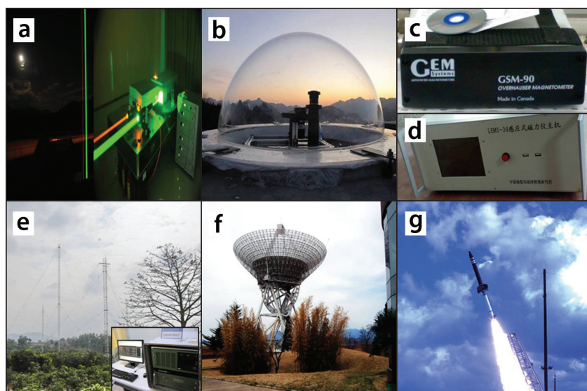
Figure 2. Examples of the observational instruments to be deployed in the Meridian Project, including (a) lidar (light detection and ranging), (b) all-sky airglow imagers, (c) Overhauser magnetometers, (d) induction magnetometers, (e) digital ionosondes (digisondes), (f) radar to monitor scintillation, and (g) sounding rockets.
